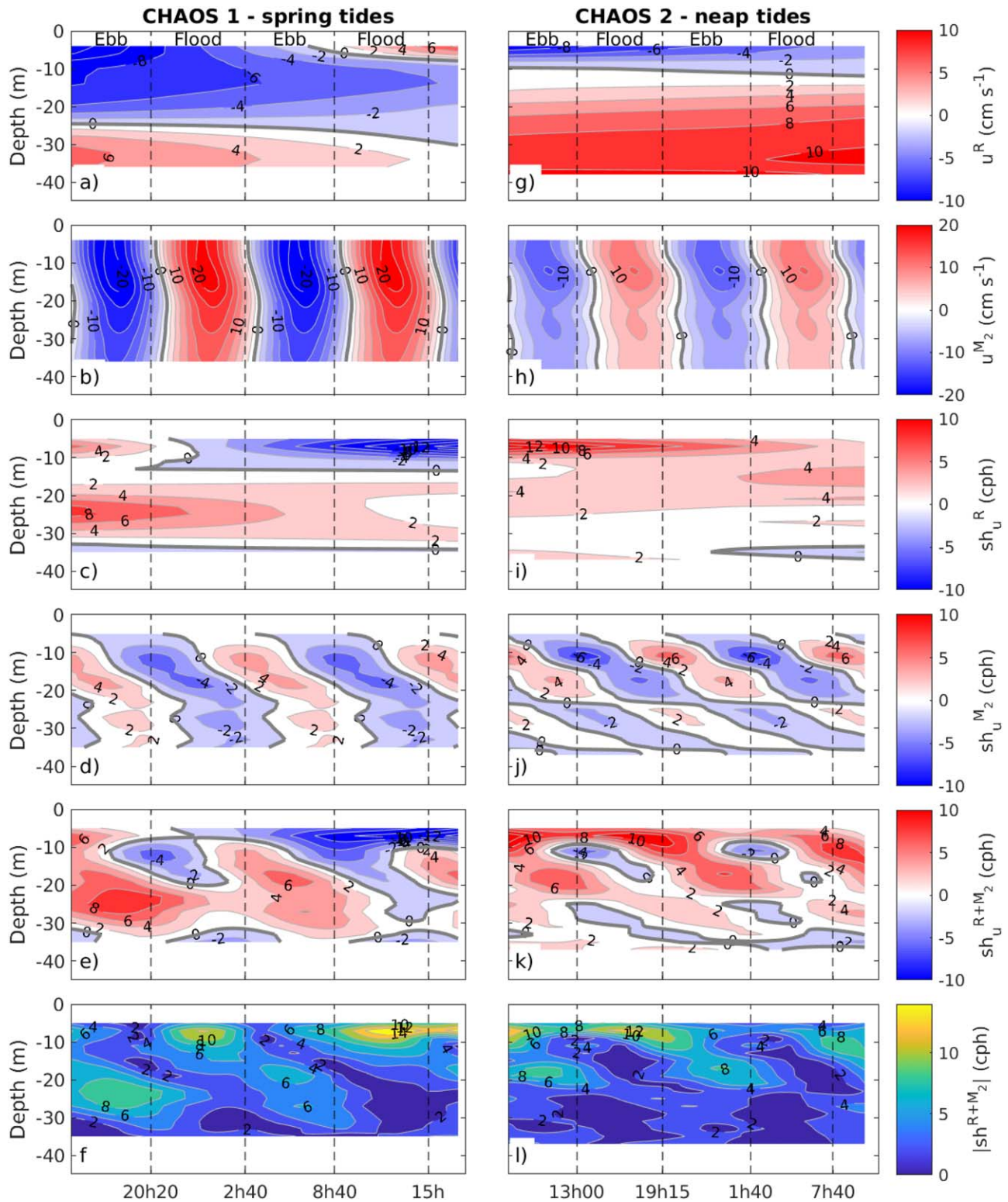
Figure 7. Currents and shear calculated in the along-Ría axis during the two intensive sampling periods at outer Ría de Vigo: CHAOS 1 - Spring tides (20–21 August 2013) and CHAOS 2 - Neap tides (27–28 August 2013). Panels (a,g) and (b,h) represent the evolution of the residual ( u^R , \text{cm s}^{-1} ) and tidal currents ( u^{M_2} , \text{cm s}^{-1} ), respectively. Panels (c,i) and (d,j) represent the shear of the residual ( sh_u^R , cph) and tidal currents, ( sh_u^{M_2} , cph), respectively, and panels (e,k) the superposition of both residual and tidal shear ( sh_u^{R+M_2} , cph). Panels (f,l) represent the magnitude, |sh^{R+M_2}| = \sqrt{(sh_u^{R+M_2})^2 + (sh_v^{R+M_2})^2} , of the total (tidal + residual) shear.
