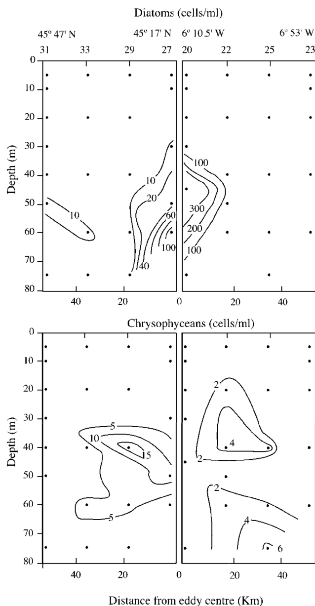
Figure 12. Vertical distribution of the abundance ( \text{cell ml}^{-1} ) of diatoms and chrysophyceans along the east–west, north–south intensive section.
