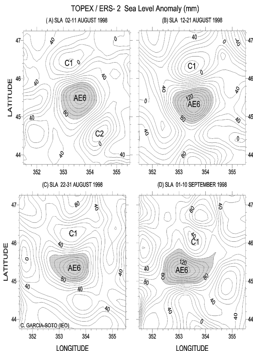
Figure 2. Maps of sea level anomaly (TOPEX-Poseidon and ERS-2 data) showing the spatial structure of swoddy AE6 on dates: (A) 02–11 August 1998; (B) 12–21 August 1998; (C) 22–31 August 1998; and (D) 01–10 September 1998. The sea level elevation associated to the anticyclonic swoddy is highlighted with shading. ‘C1’ and ‘C2’ indicate surrounding cyclones.
