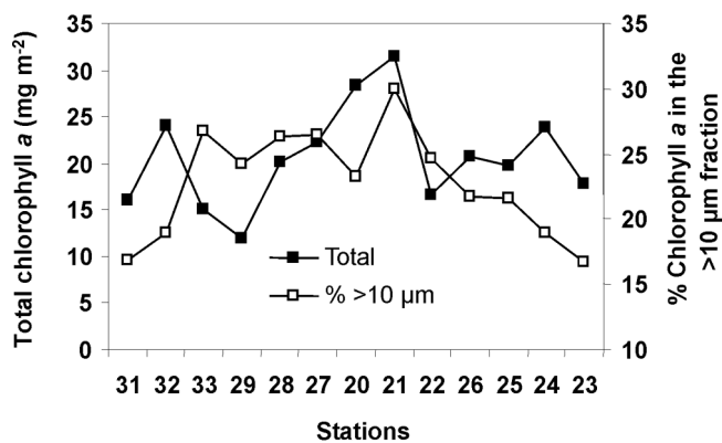
Figure 11. Spatial distribution of depth integrated chlorophyll- a (100 m) and the relative contribution of >10 µm phytoplankton cells to total chlorophyll- a along the east-west, north-south intensive section.
