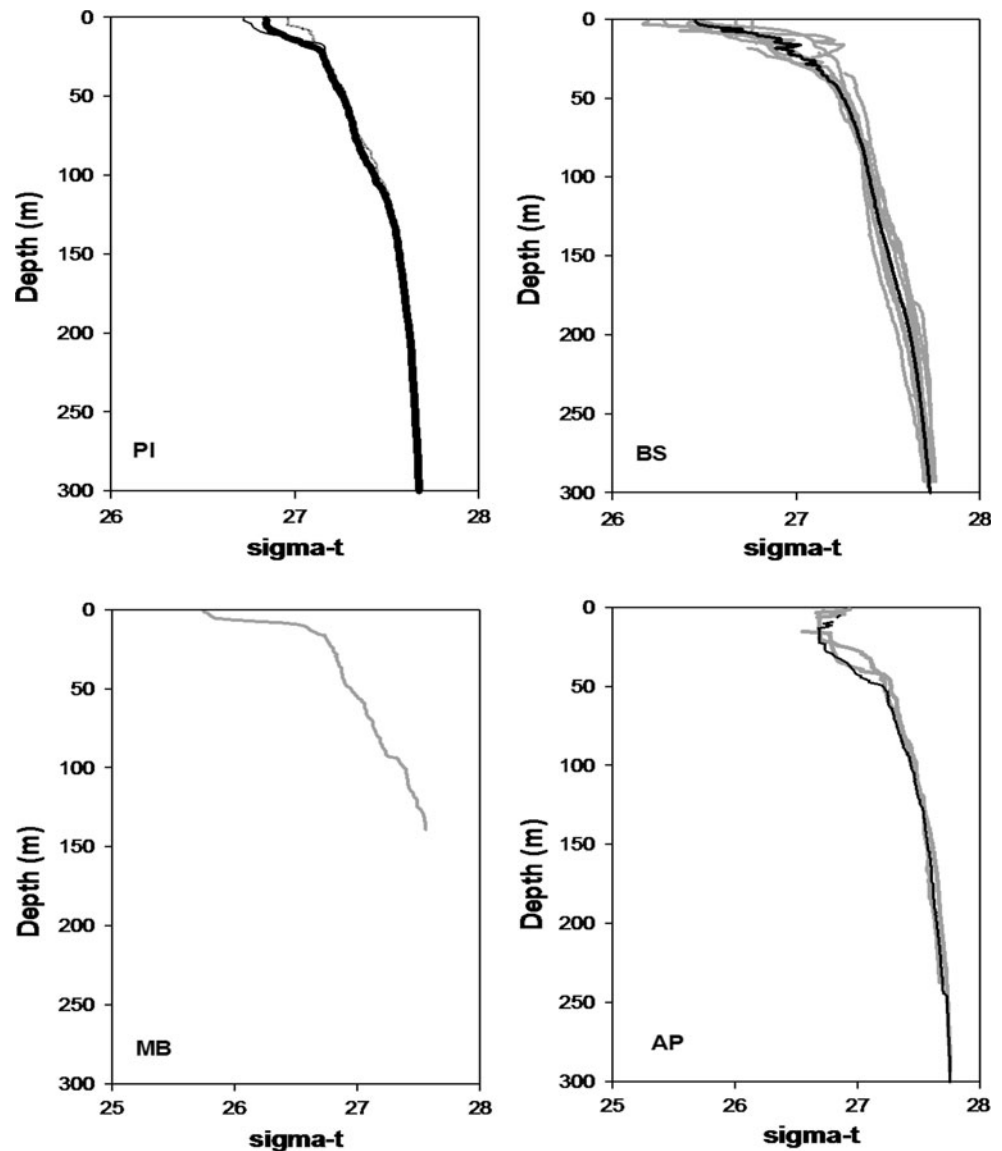
Fig. 3 Vertical profiles of density anomaly ( \sigma\text{-}t ) for the stations sampled in the Antarctic Peninsula (AP), Marguerite Bay (MB), the Bellingshausen Sea (BS) and Peter I Island (PI), in January–February 2006. \sigma\text{-}t is the density anomaly of a water sample when the total pressure on it has been reduced to atmospheric pressure (i.e. zero water pressure), and temperature and salinity correspond to in situ values. Thick dark line represents the averaged profile for all stations sampled in each region
